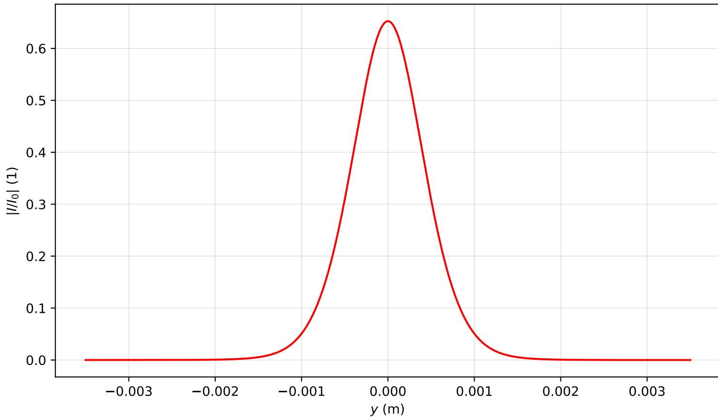
Intensity profile I(x = 0, y, z = 2.627)/I_0 , P_{in}=0.5P_{cr} , artificial time
